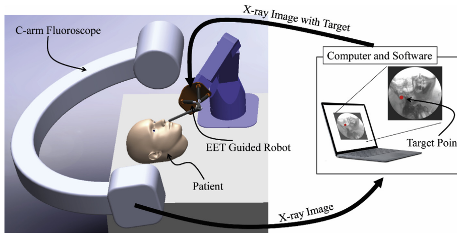
Figure 3 Conceptual design of EET guided robotic system with robot diagram.
