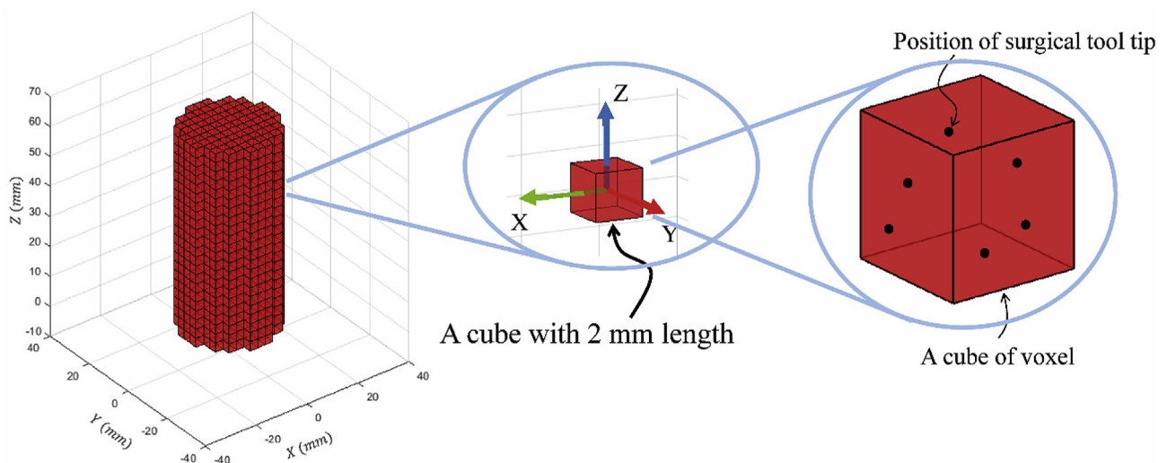
Figure 2 Voxelization method of EET cloud position.
