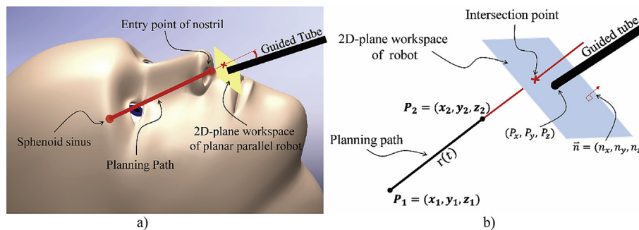
Figure 4 a) Automatic operation of guiding robot and b) Mathematical diagram of automatic operation.
