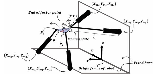
Figure 5 Mechanism of EET guiding robot.
