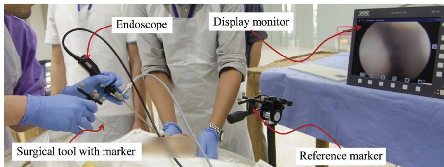
Figure 8 EET experiment on cadaver.
