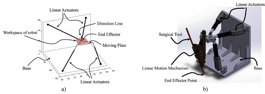
Figure 6 Simulation of the EET guiding robot with workspace determination.
