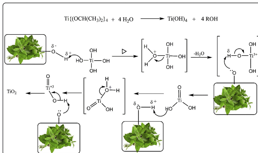
Fig. 3. Possible reaction mechanism for the formation of \text{TiO}_2 NPs in presence of hydroxyl group (-OH) of leaf extract of Origanum majorana as a capping agent.
