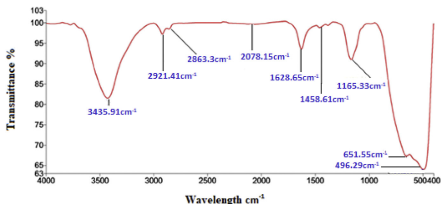
Fig. 4. FT-IR of \text{TiO}_2 nanoparticles synthesized using leaf extract.
