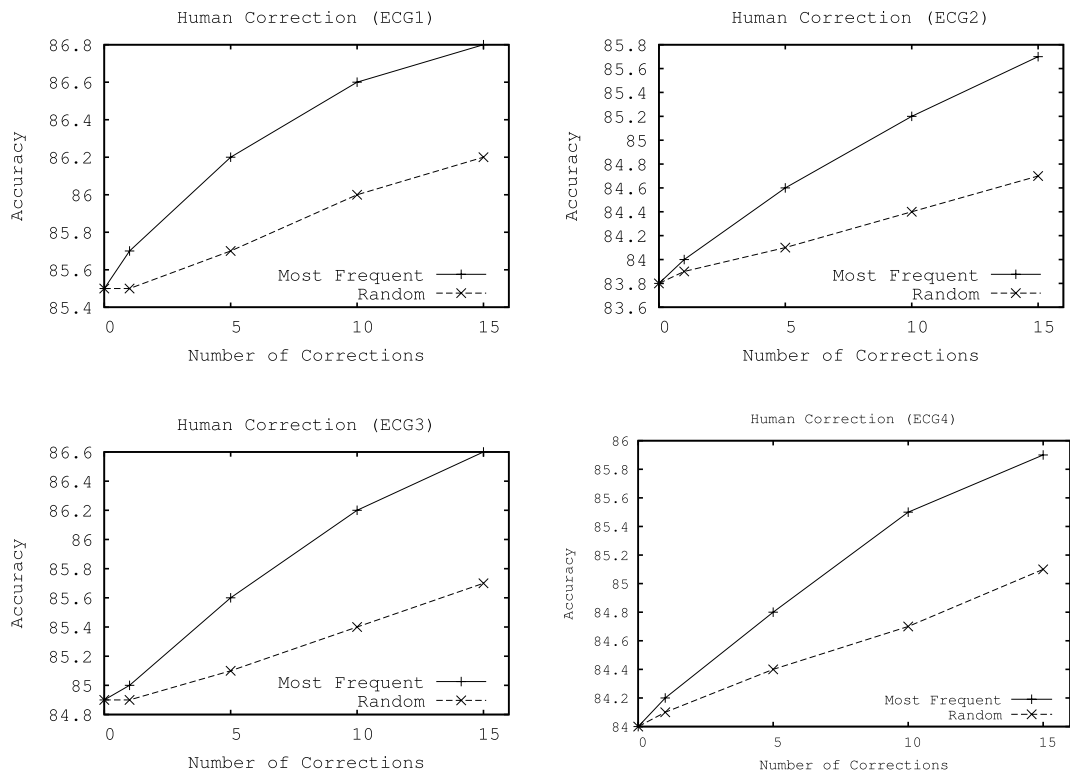
Fig. 15. Extraction accuracy with human annotated correction.
