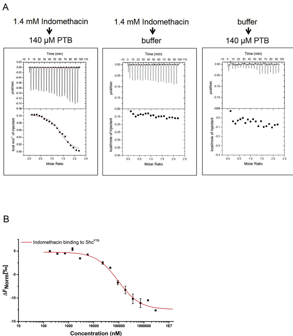
Fig. 2. Direct interaction of indomethacin and Shc PTB . (A) ITC measurement of the interaction between Indomethacin and Shc PTB . Left: Twenty 15 \mu l injections of indomethacin (1400 \mu M) were titrated into Shc PTB (140 \mu M) at 25 °C. Top panel: baseline-corrected power versus time plot for the titration. Bottom panel: the integrated heats and the molar ratio of the indomethacin to Shc PTB . Middle: the heats of dilution of 1400 mM indomethacin titrated into buffer. Right: the heats of dilution of buffer titrated into Shc PTB (140 \mu M). (B) Interaction of indomethacin with Shc PTB is measured using MST. Unlabelled indomethacin (2.9 \mu M–178 nM) was titrated into a fixed concentration of labelled Shc PTB (50 nM).
