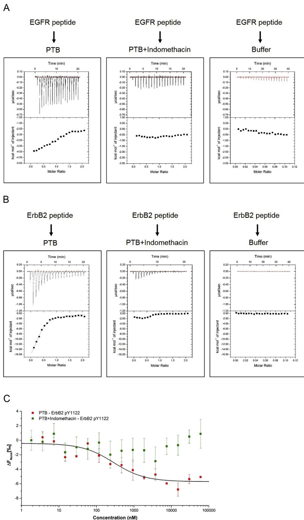
Fig. 4. Binding of indomethacin to Shc PTB reduces the Shc PTB –phosphotyrosine interaction. (A) ITC measurement of the interaction between EGFR pY1148 (EGFR peptide: STAVGNPEpYLNT) and Shc PTB in the absence and presence of indomethacin. Left: twenty 2 \mu l injections of EGFR pY1148 (500 \mu M) were titrated into Shc PTB (50 \mu M) at 25 ^{\circ} C. Middle: twenty 2 \mu l injections of EGFR pY1148 (500 \mu M) were titrated into 50 \mu M Shc PTB pre-incubated with 2 mM of Indomethacin at 25 ^{\circ} C. Right: control experiment in which twenty 2 \mu l injections of EGFR pY1148 (500 \mu M) were titrated into buffer solution. (B) ITC measurement of the interaction between ErbB2 pY1122 (SPAFDNLYpYWDQ) and Shc PTB in the absence and presence of indomethacin. Left: twenty 2 \mu l injections of ErbB2 pY1122 (500 \mu M) were titrated into Shc PTB (50 \mu M) at 25 ^{\circ} C. Middle: twenty 2 \mu l injections of ErbB2 pY1122 (500 \mu M) were titrated into 50 \mu M Shc PTB pre-incubated with 2 mM of indomethacin at 25 ^{\circ} C. Right: Control experiment in which twenty 2 \mu l injections of EGFR pY1148 (500 \mu M) were titrated into buffer solution. (D) Interaction of indomethacin with Shc PTB is measured using MST. Unlabelled ErbB2 pY1122 (60 \mu M–1.83 nM) was titrated into a fixed concentration of labelled Shc PTB (50 nM) (red curve). Pre-incubated Shc PTB (50 nM) with 200 \mu M indomethacin disrupted the interaction to ErbB2 pY1122 peptide (green curve). (For interpretation of the references to colour in this figure legend, the reader is referred to the Web version of this article.)
