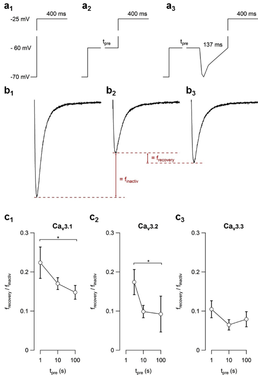
Fig. 3. Slowing of recovery reduces T-type \text{Ca}^{2+} channel availability following IPSPs. T-type \text{Ca}^{2+} channels were activated with a depolarizing voltage step to -25 mV (panel a 1 , representative current trace in a 1 ). Subsequently, channel availability was measured following a depolarizing step (1–100 s) to -60 mV (panel a 2 ) to determine the inactivated fraction (panel b 2 ). Finally, the same inactivating voltage step was applied followed by a mock IPSP and the test-pulse to -25 mV (panel a 3 ). The recovering fraction was defined as the increase of the current amplitude compared to panel b 2 (see panel b 3 ). This fraction was normalized to the inactivated fraction and plotted versus the duration of the inactivating stimulus (panel c 1 –c 3 , n \leq 7 ). Prolonged depolarization slows down the recovery (see Fig. 2) resulting in a smaller fraction recovering during the IPSP for \text{Ca}_V3.1 and \text{Ca}_V3.2 channels (panel c 1 and c 2 , significant when comparing 1 s to 100 s, indicated by asterisks). For \text{Ca}_V3.3 the recovering fraction was independent of the prepulse duration (panel c 3 ).
