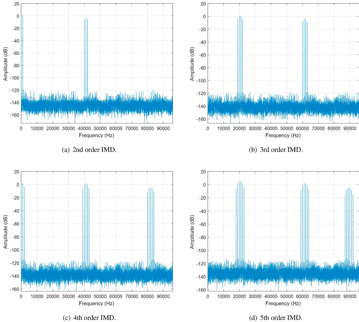
Figure A.30. Simulated spectrum of the 2nd to 5th order IMD for (f_1, f_2) = (20 \text{ kHz}, 21 \text{ kHz}) .
