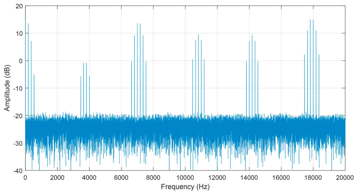
Fig. 14. Simulated cumulative audible spectrum of 2nd through 7th order IMD for 25 kHz, 32 kHz, and 32.18 kHz tones.
