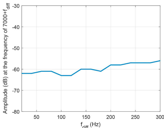
Fig. 25. The amplitude of IMD product at different frequencies.
