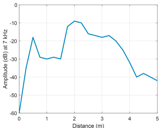
Fig. 28. The amplitude of the IMD product at 7 kHz at different distances.
