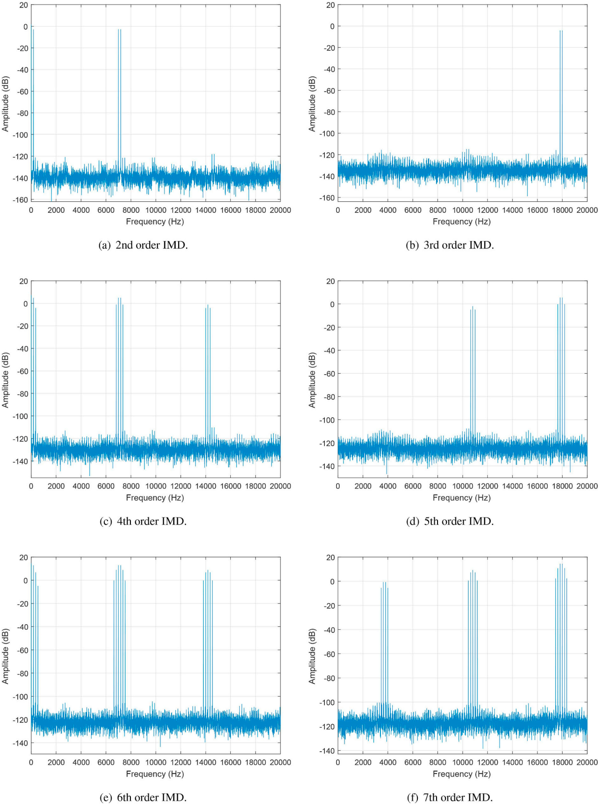
Figure A.31. Simulated audible spectrum of the 2nd to 7th order IMD for 25 kHz, 32 kHz, and 32.18 kHz tones.2
