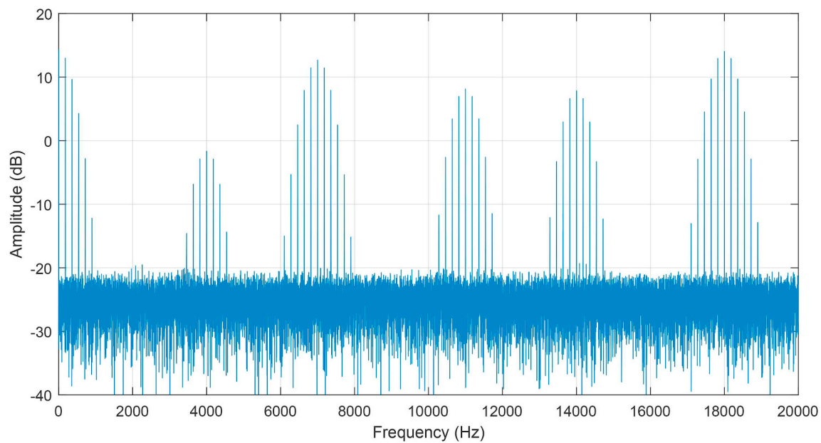
Fig. 16. Simulated cumulative audible spectrum of 2nd through 7th order IMD for 25 kHz tone and 180 Hz AM modulated over a 32 kHz carrier.
