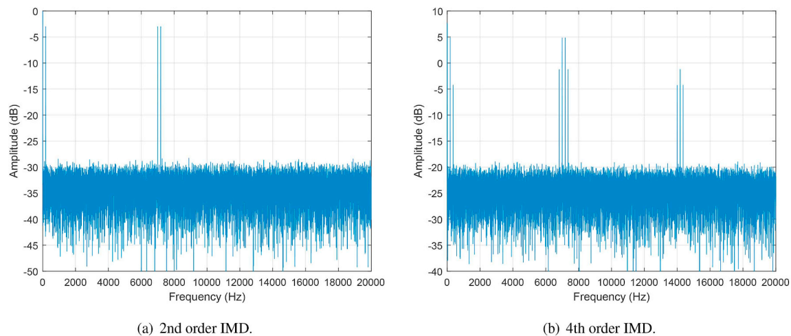
Fig. 13. Simulated audible spectrum of the 2nd (a) and 4th order IMD (b) for 25 kHz, 32 kHz, and 32.18 kHz tones.
