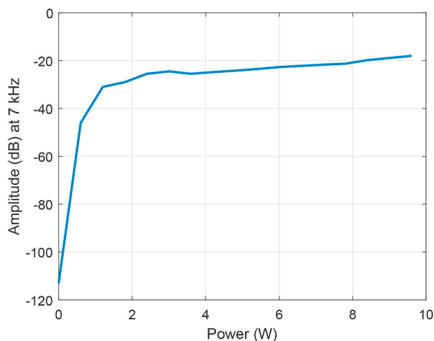
Fig. 27. The amplitude of the IMD product at 7 kHz with different emitting powers.
