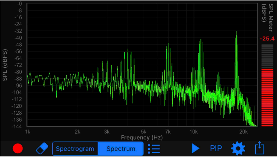
Fig. 21. Spectrum of sounds heard by a smartphone when playing 25 kHz and 180 Hz AM modulated on a 32 kHz carrier. The IMD spectrum resembles the ripples near 7 kHz in the AP news spectrum.
