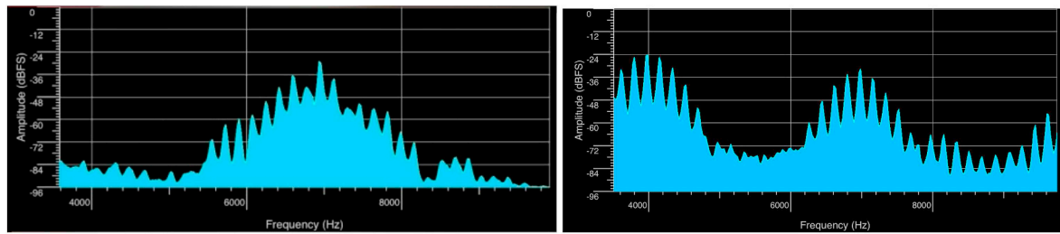
Fig. 23. The spectra from the AP news (L) and one of our experiments (R).
