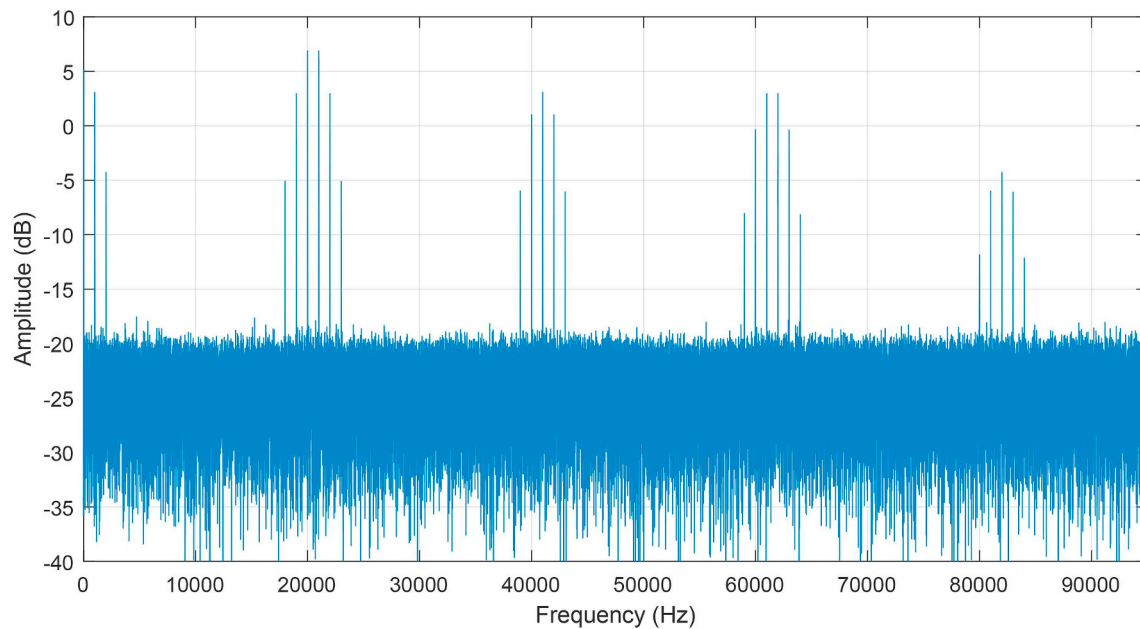
Fig. 12. Simulated cumulative audible spectrum of 2nd through 5th order IMD for 20 kHz and 21 kHz tones.
