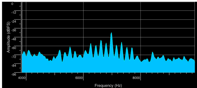
Fig. 24. The spectrum from one of our experiments showing only signals around 7 kHz.
