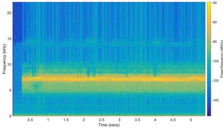
Fig. 10. The spectrogram-time plot (waterfall) of metallic sounds extracted from the AP news video.
