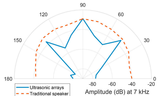
Fig. 29. The amplitude of the IMD product at 7 kHz and a sound played by a traditional speaker at different angles.
