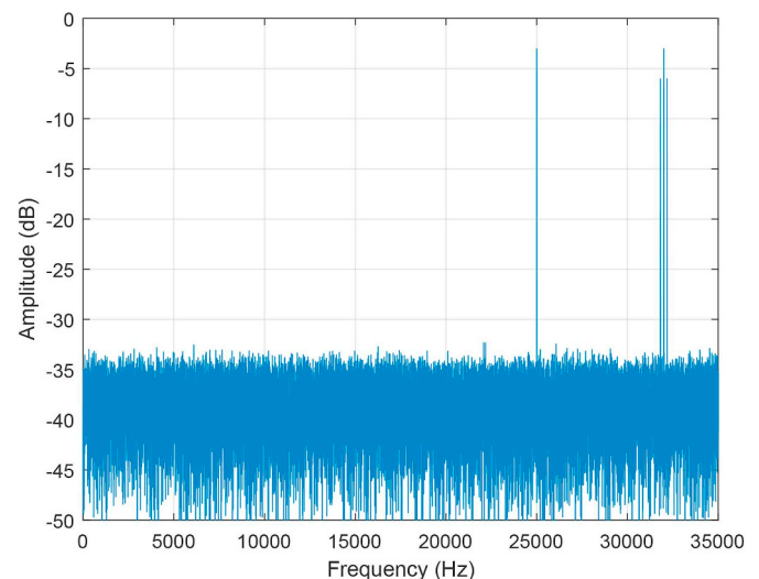
Fig. 15. Simulated spectrum of 25 kHz tone and 180 Hz AM modulated over a 32 kHz carrier.
