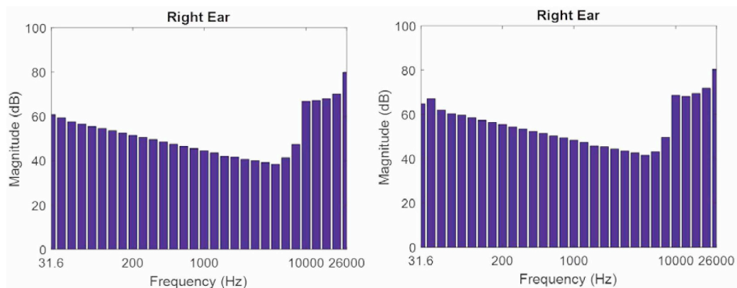
Fig. 2. 1/3 octave spectrum for 60 s (left) and 1 s (right) noise signals generated by a Zoonic pest repeller at the high frequency setting. (Courtesy of Dr. Jun Qin at Southern Illinois University Carbondale).
