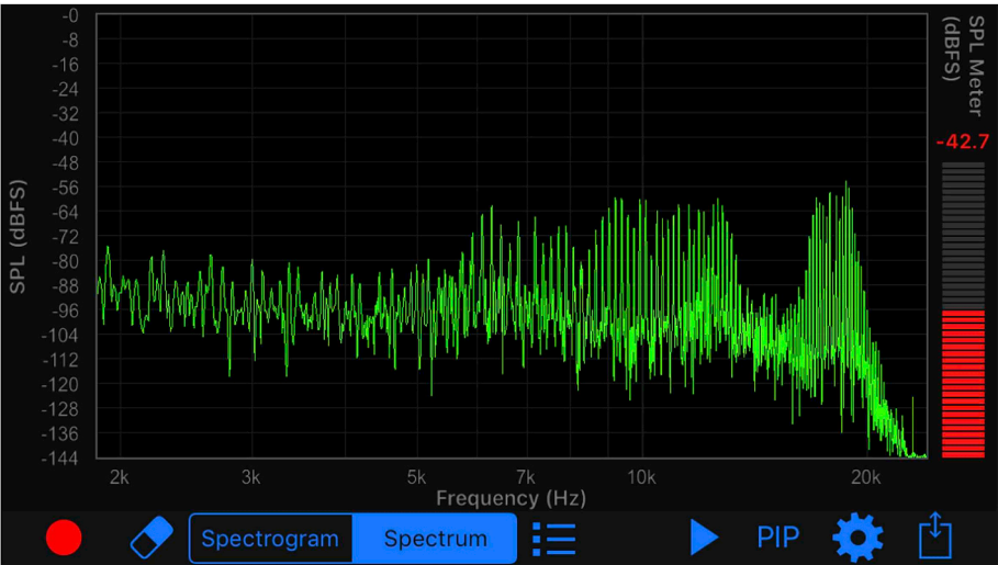
Fig. 22. Spectrum of sounds heard by a smartphone when playing 25 kHz and 180 Hz FM modulated on a 32 kHz carrier.
