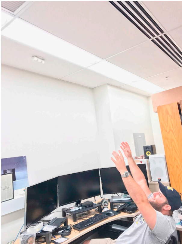
Fig. 1. Many offices contain ultrasonic emitters in the ceiling to determine room occupancy for controlling lights. The offices at the University of Michigan use a continuous 25 kHz ultrasonic tone. Computer Science & Engineering Ph.D. student Connor Bolton notices one such unwanted, inaudible ultrasonic emitter.
