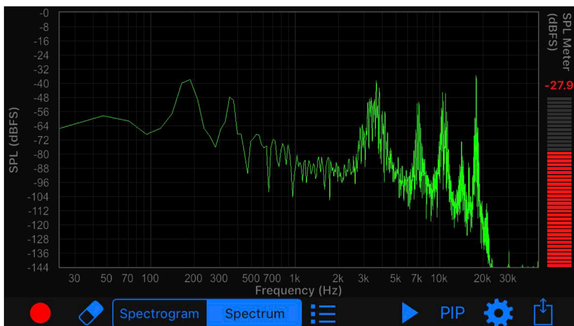
Fig. 18. Spectrum recorded during an IMD experiment playing three ultrasonic tones (25 kHz, 32 kHz, 32.18 kHz).
