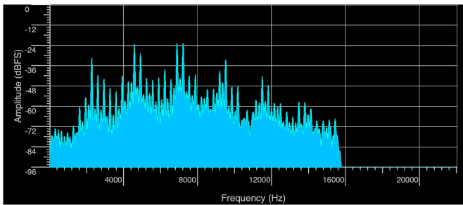
Fig. 7. The spectral analysis of sounds from cicadas contains energy near 7 kHz, but without evidence of localization.
