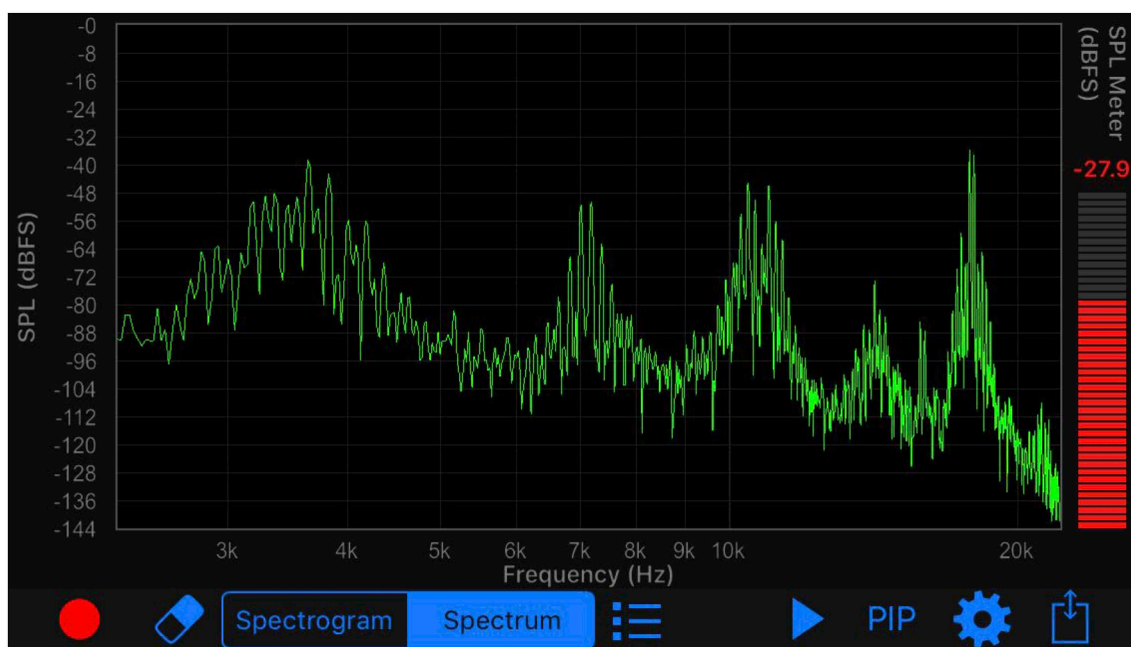
Fig. 19. Magnified spectrum of the signals near 7 kHz during an IMD experiment playing three ultrasonic tones (25 kHz, 32 kHz, 32.18 kHz).
