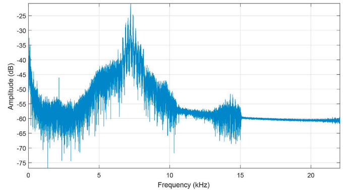
Fig. 9. The spectrum of metallic sounds extracted from the AP news video. The spectrum of the AP news audio ends abruptly at 15 kHz. We suspect this is an artifact of either the AP audio filtering, YouTube audio filtering that is known to roll off beginning at 16 kHz, or iPhone audio filtering that begins to roll off at 21 kHz on our equipment.
