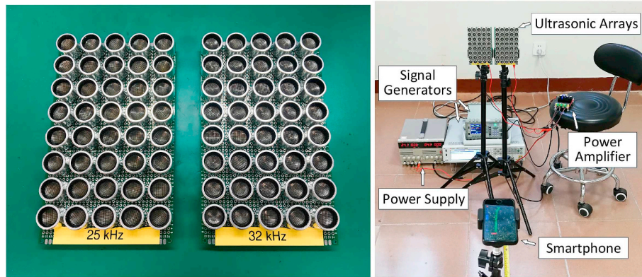
Fig. 26. The ultrasonic transducer arrays (L) that are capable of transmitting high-power ultrasounds at 25 kHz and 32 kHz, and the experiment setup (R) with the arrays.
