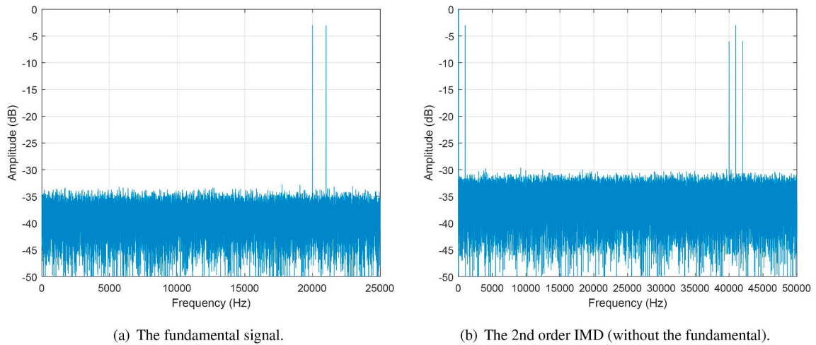
Fig. 11. Simulated spectra of (a) a fundamental signal with pure tones at 20 kHz and 21 kHz, and (b) its 2nd order IMD derivative (which will be added on top of the original fundamental signal) after passing a nonlinear equation in MATLAB.
