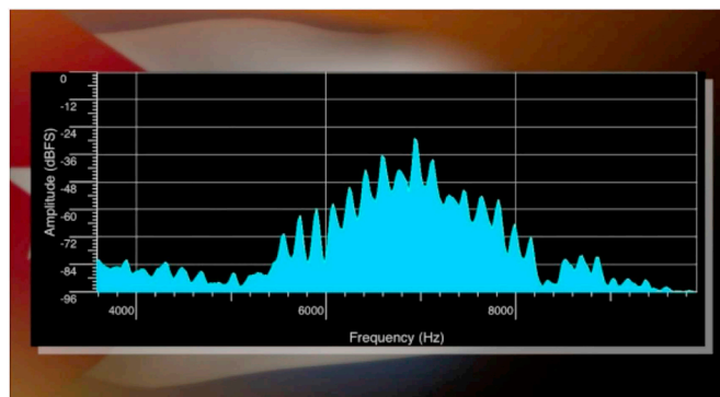
Fig. 5. Screen shot of the AP news showing the Fourier transform of what was reported as sounds heard by diplomats in Cuba.
