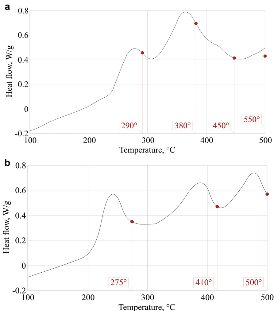
Fig. 2. The results of investigation of multilayer structures with an excess of aluminum (a) and nickel (b) by the DSC method.
