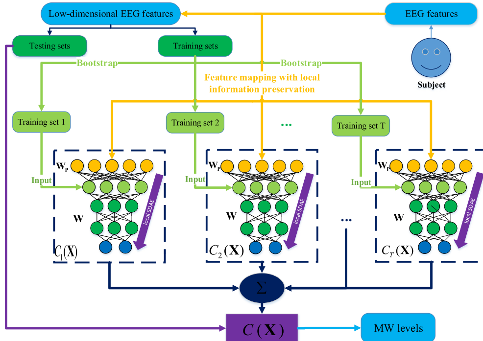
Fig. 3. Architecture of the EL-SDAE model.
