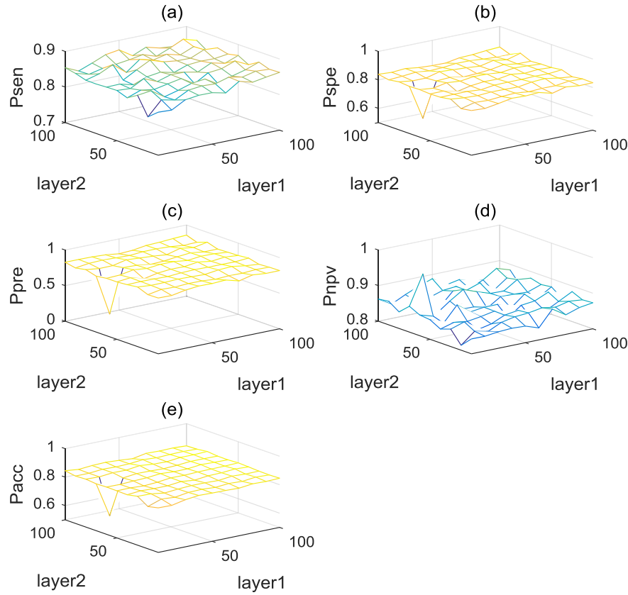
Fig. 5. Model selection of the member SDAE with a two-hidden-layer deep structure.
