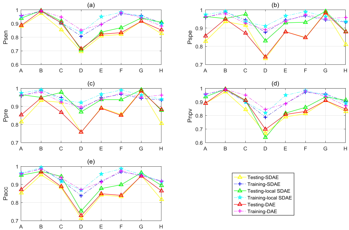
Fig. 8. Comparison of training and testing classification performance indices of different base learners in EL-SDAE.
