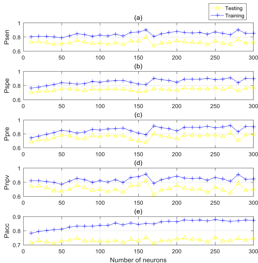
Fig. 9. Participant-average MW classification performance vs. the number of hidden neurons in a SDAE model.
