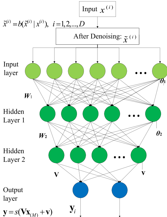
Fig. 2. Architecture of SDAE for EEG modeling.
