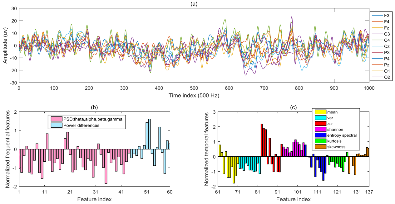
Fig. 1. Filtered EEG data in (a) a 2 s segment of 11 channels, (b) the corresponding 60 frequential features and (c) the corresponding 77 temporal features. Power spectral density, variance, and zero crossing rate are denoted by PSD, var, and zcr in the legend, respectively.
