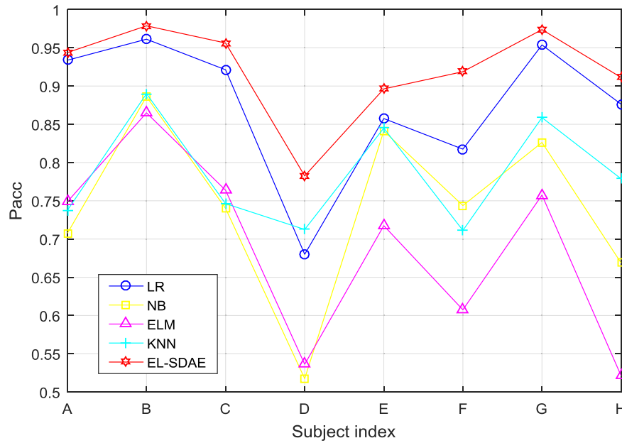
Fig. 6. Classification accuracy comparison between EL-SDAE and shallow MW classifiers.
